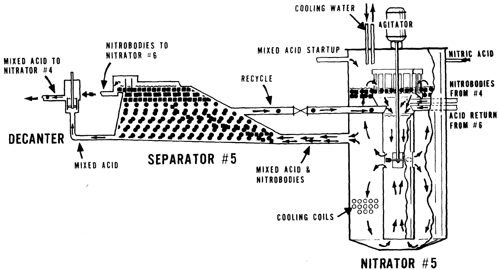
Fig 2 (from Ref 38) TNT Nitrator System
